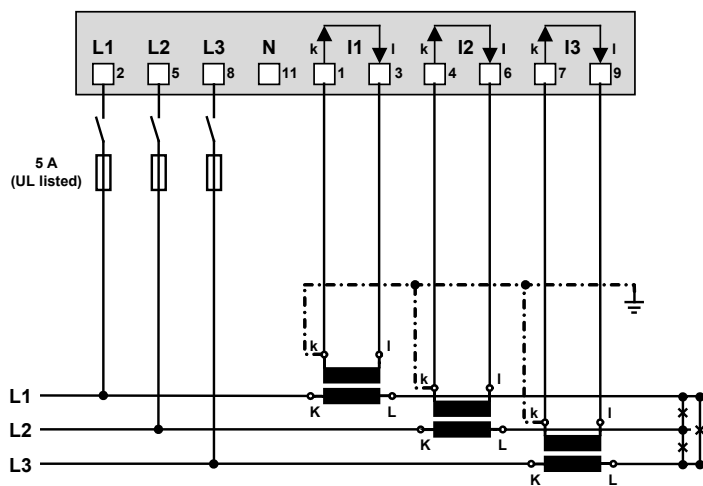
With current transformers
