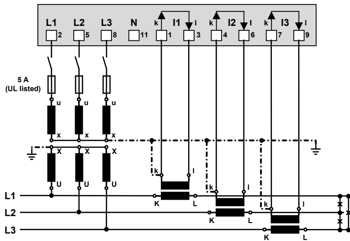
With current and 3 single-pole isolated voltage transformers
