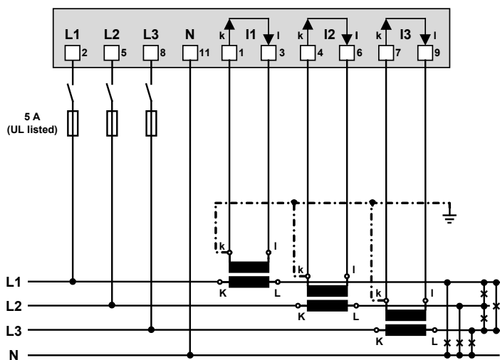
With current transformer
