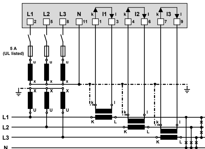
With current and 3 single-pole isolated voltage transformers
